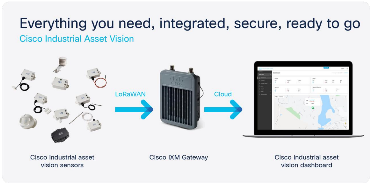
Figure 1. Cisco Industrial Asset Vision components
