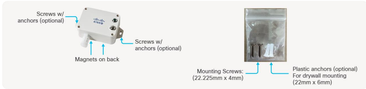
Figure 13. Mounting Accessories and Methods AV203
