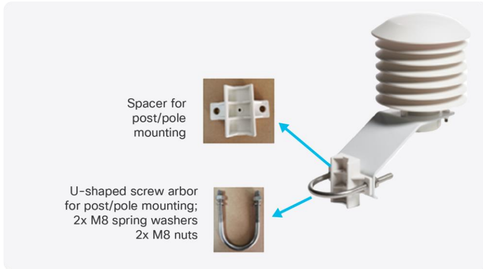
Figure 4. Mounting Accessories and Methods AV200
