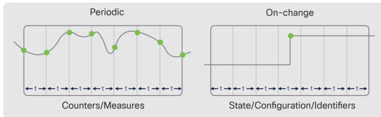
Figure 80. 234AGRAM Periodic vs. On-Change subscriptions
