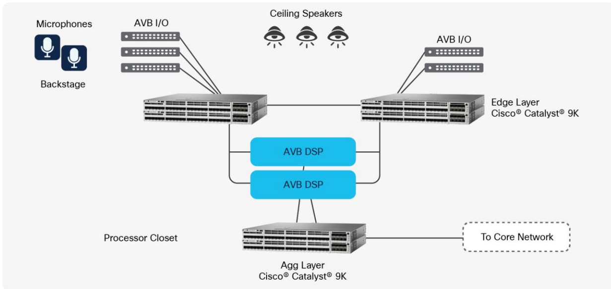
Figure 66. AVB Network
