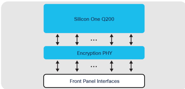
Figure 14. Cisco Catalyst 9500X switch block diagram – Cisco Silicon One Q200
