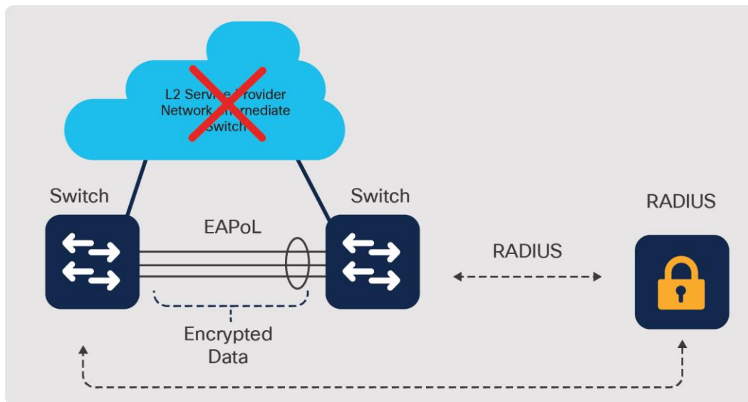
Figure 45. Switch-to-switch MACsec encryption
