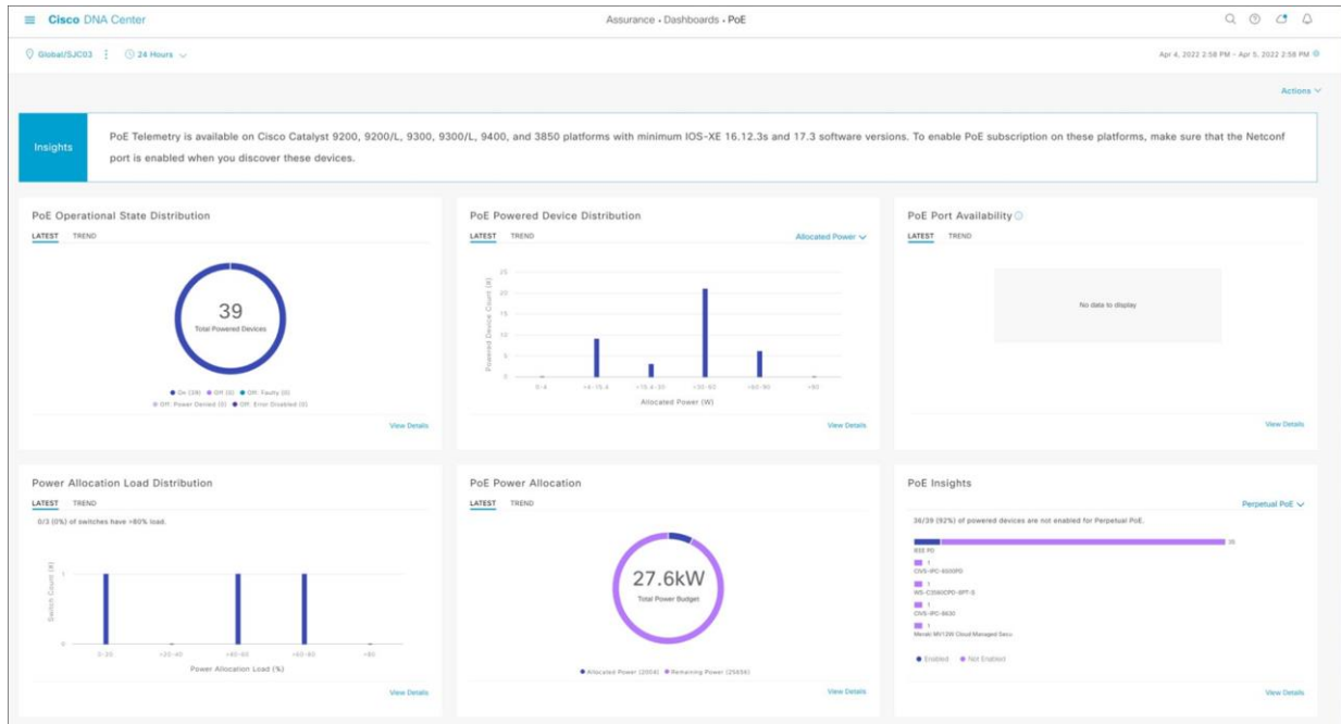
Figure 70. Cisco DNA Center – Power Assurance
